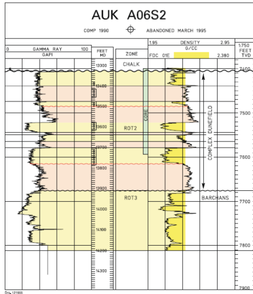
Fig. 7. Typelog for the Rotliegend unit 2 reservoir and Rotliegend unit 3 aquifer, yellow indicates net reservoir whilst orange-brown indicates waste zones. The Rotliegend unit 1 and the Zechstein is eroded in this well.
