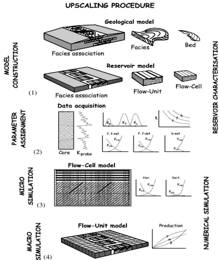
Fig. 1. Schematic representation of the four-step upscaling procedure of this work. Step 1: Model construction, consisting of geological and reservoir model and assignment of its elements. Step 2: Parameter assignment, consisting of permeability sampling, data analysis, and calculation of relative permeability and capillary pressure. Step 3: Micro-simulation, consisting of numerical flow simulation on all flow cell models of the reservoir, yielding effective 1- and 2-phase permeabilities, and capillary pressures. Step 4: Macro simulation consisting of numerical flow simulation on the entire reservoir, yielding production history. Steps 1 and 2 form reservoir characterisation. Steps 3 and 4 form numerical flow simulation. K_c , K_f , K_b , are permeabilities of coarse, fine foreset, and bottomset, resp. K_{rc} , K_{rf} , K_{rb} are relative permeabilities of oil and water, resp. C, F, B stand for coarse-, fine foreset and bottomset.
