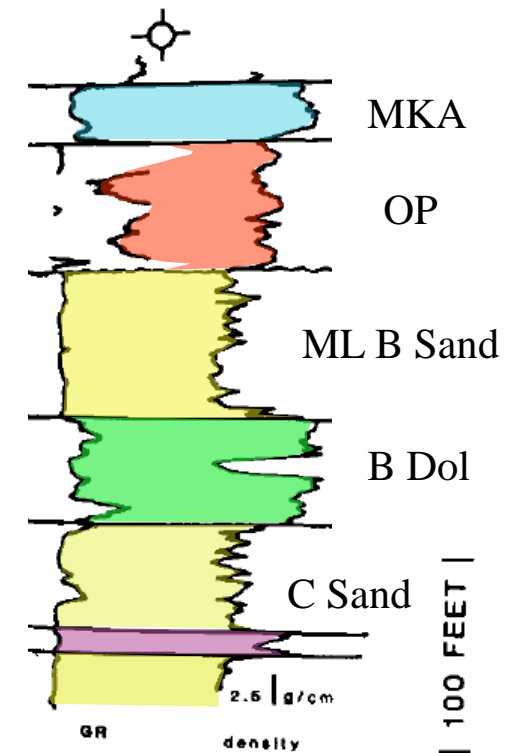
GR-Sonic logs from a Minnelusa well in the play area opposite the outcrops. After Fryberger, 1984
