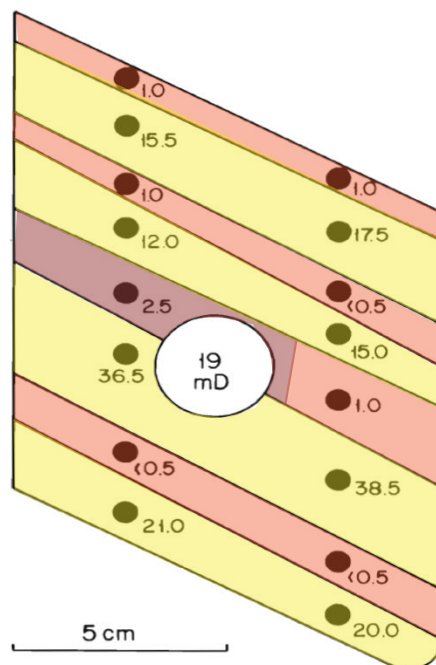
FIG. 17.—Aeolian core slab with a dense grid of mini-permeameter permeability readings. Aeolian crossbed set boundaries are indicated.
