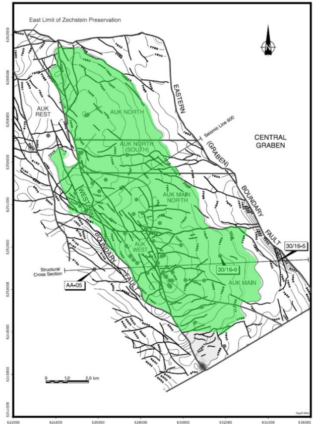
Top Rotliegendes structure map and well locations, Auk field. The Zechstein is only preserved in the west part of the field, towards the east Early Cretaceous erosion has removed all of the Zechstein, and cut into the Rotliegendes reservoir.
