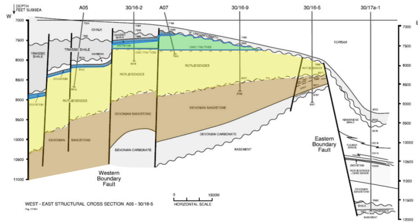
Geological cross section in W-E direction through Auk Main block and into the Central North Sea Graben, illustrating the trapping of hydrocarbons to the west against Aptian shales.
