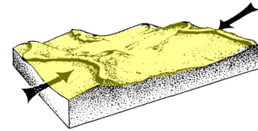
Reversing
