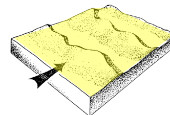
Barchanoid ridge
