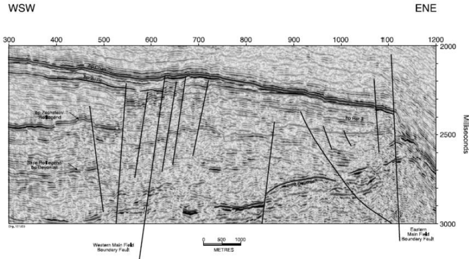
Seismic cross section in SW-NE direction through Auk Main North block.
