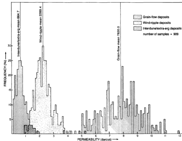
Figure 4—Histogram showing Page Sandstone permeability data. See discussion in text.
