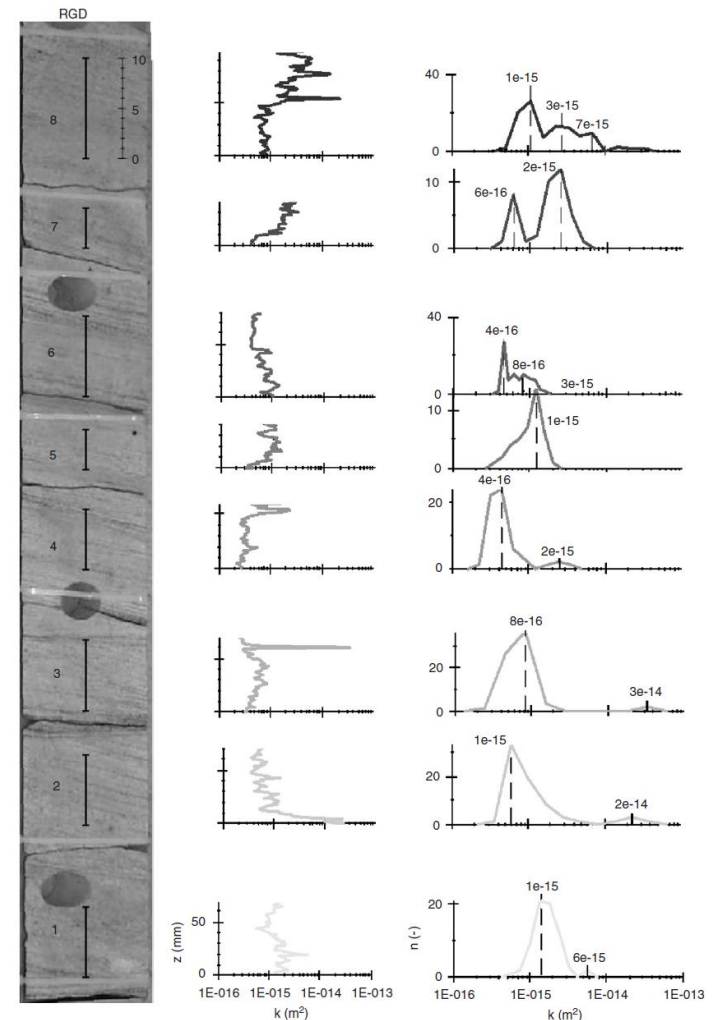
Fig. 10. Permeability curves from core RGD. Curves show different values, contrasts and trends and PDFs show different modes and shapes, ranging from unimodal symmetrical to skewed and from bimodal to trimodal. Permeability covers two orders of magnitude. Numbers indicate core sections, naturally separated along bottomsets. Black lines indicate sample profiles, sample spacing is 1 mm.
