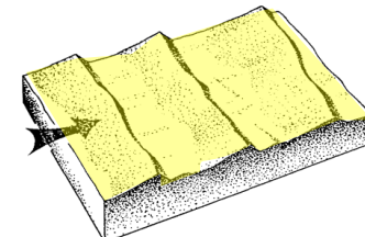
Transverse ridge
